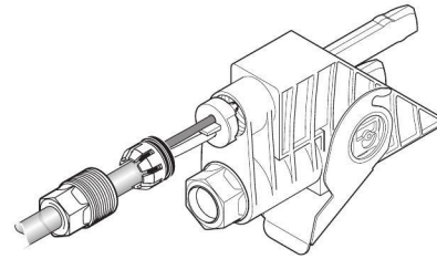
Figure 27 Bus connector
