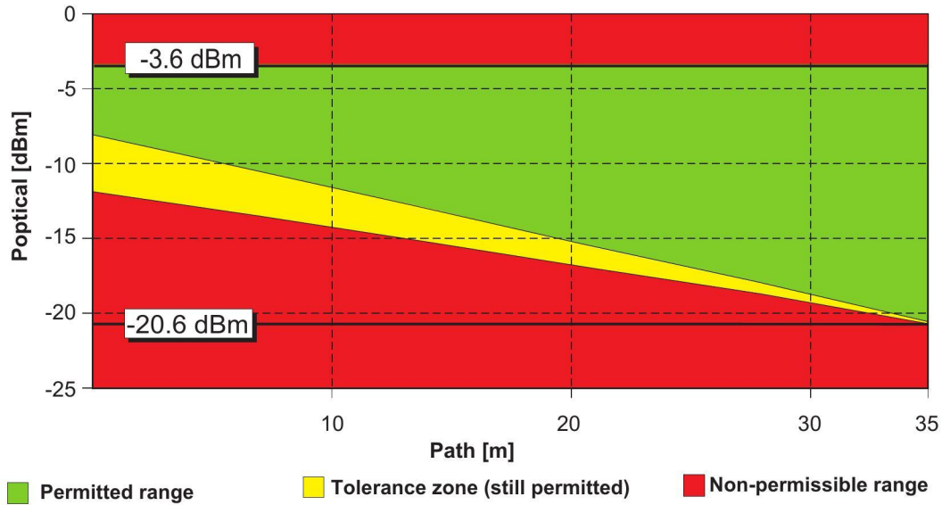
Limit Values for Polymer Fibers in Drag Chain Applications of Different Lengths (50 m System)
