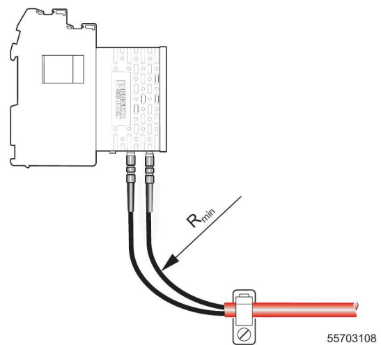
Figure 10 Secure the bending radius
