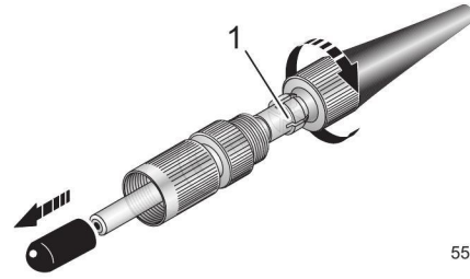
Figure 34 Unscrewing the connector (with the example of an F-SMA connector)
