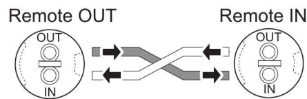
Figure 26 Crossing the individual fibers
