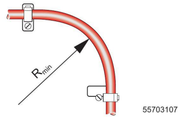
Figure 9 Maintain minimum bending radius
