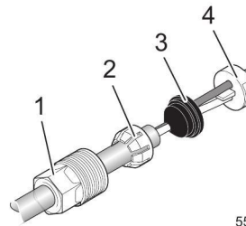
Figure 25 Individual parts
