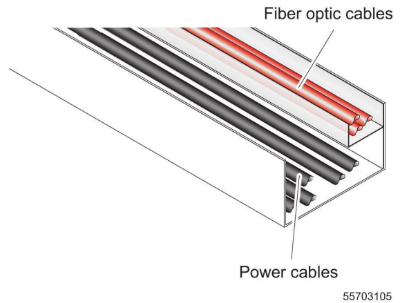
Figure 7 Separate cable ducts (example)
